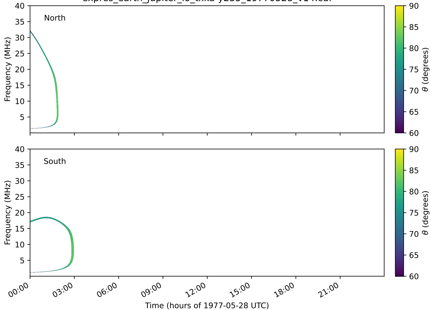
expres_earth_jupiter_io_txka-y235_19770528_v14.cdf
