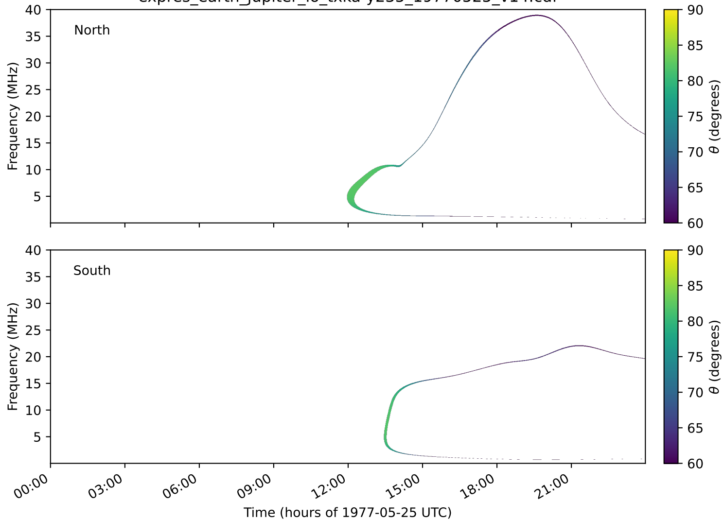
expres_earth_jupiter_io_txka-y235_19770525_v14.cdf
