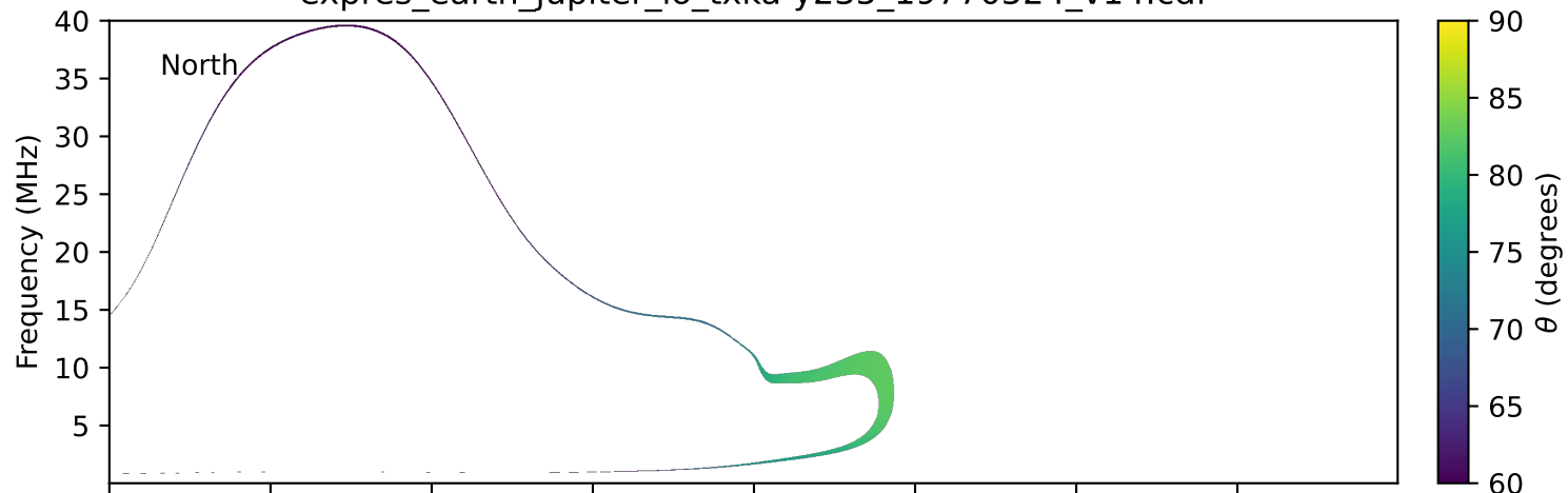
expres_earth_jupiter_io_txka-y235_19770524_v14.cdf
