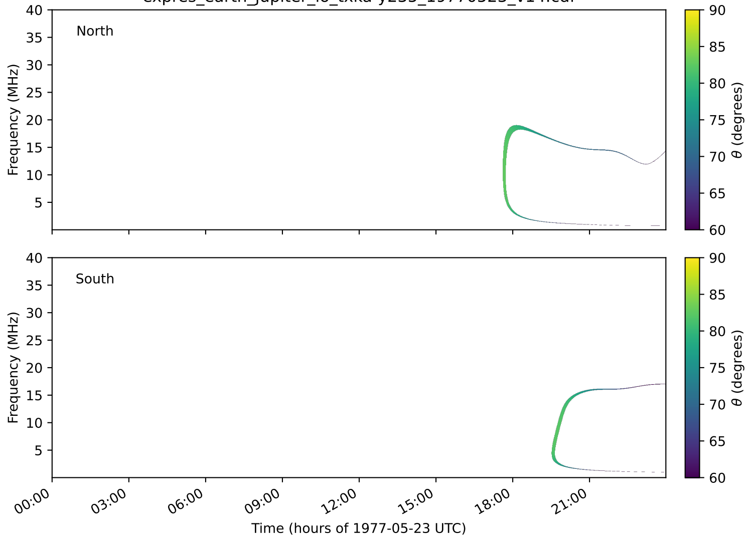
expres_earth_jupiter_io_txka-y235_19770523_v14.cdf
