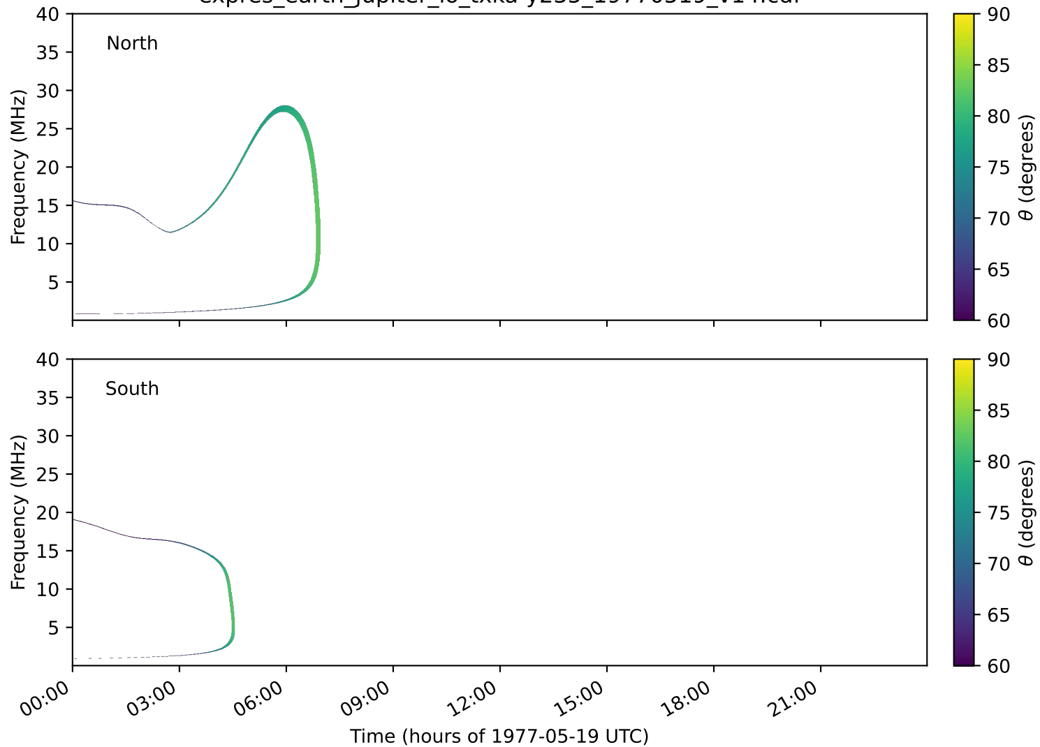
expres_earth_jupiter_io_txka-y235_19770519_v14.cdf
