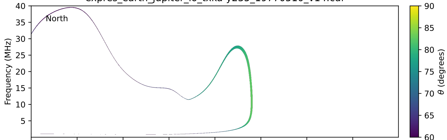
expres_earth_jupiter_io_txka-y235_19770510_v14.cdf
