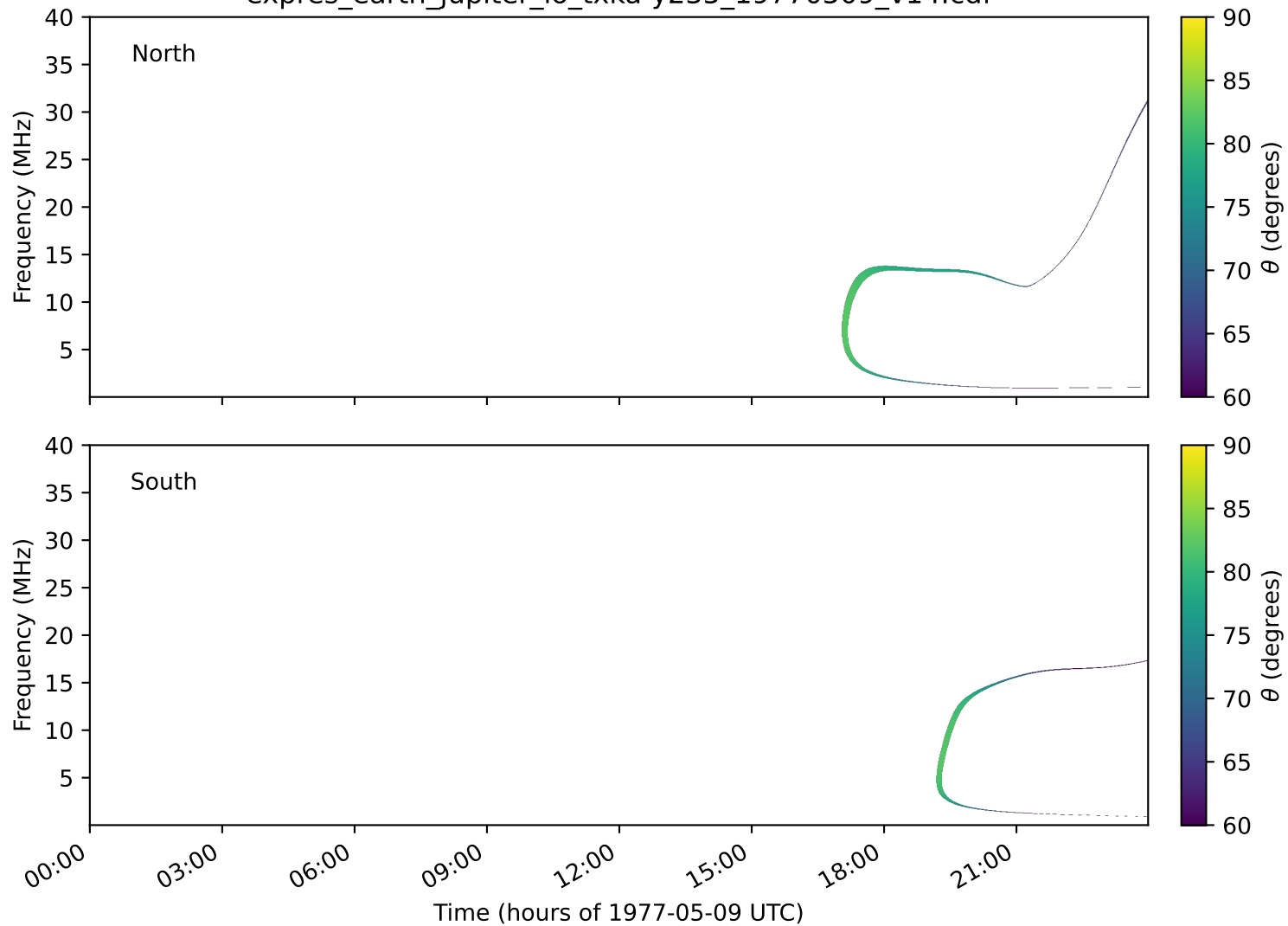
expres_earth_jupiter_io_txka-y235_19770509_v14.cdf
