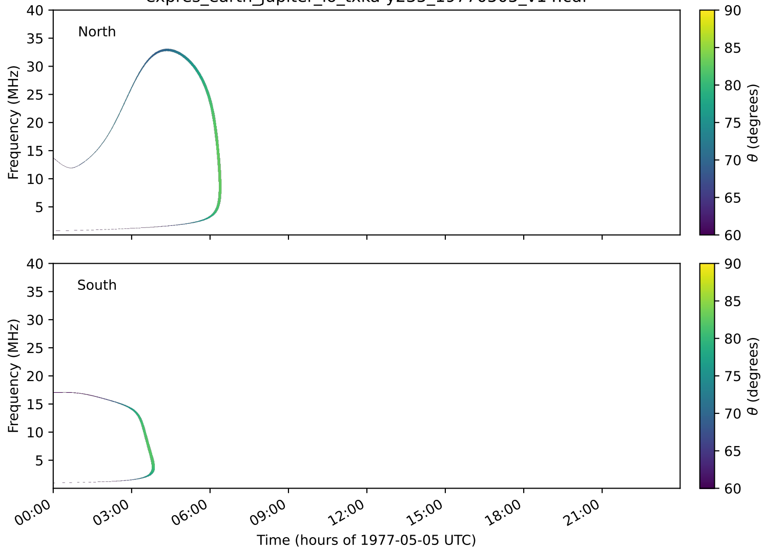
expres_earth_jupiter_io_txka-y235_19770505_v14.cdf
