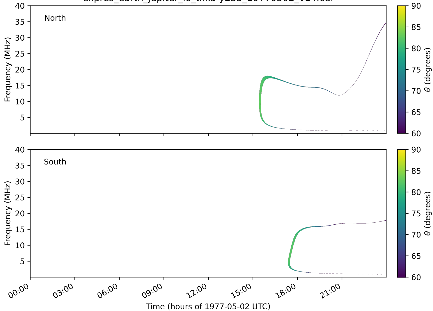
expres_earth_jupiter_io_txka-y235_19770502_v14.cdf
