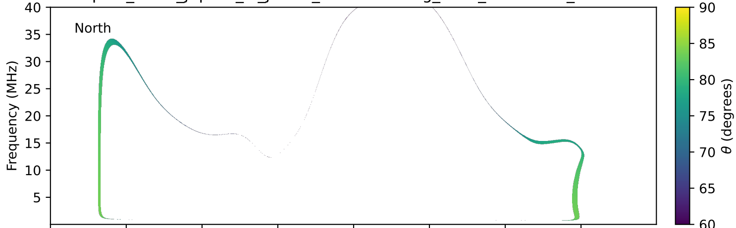
expres_earth_jupiter_io_jrm33_lossc-wid1deg_3kev_19770529_v11.cdf
