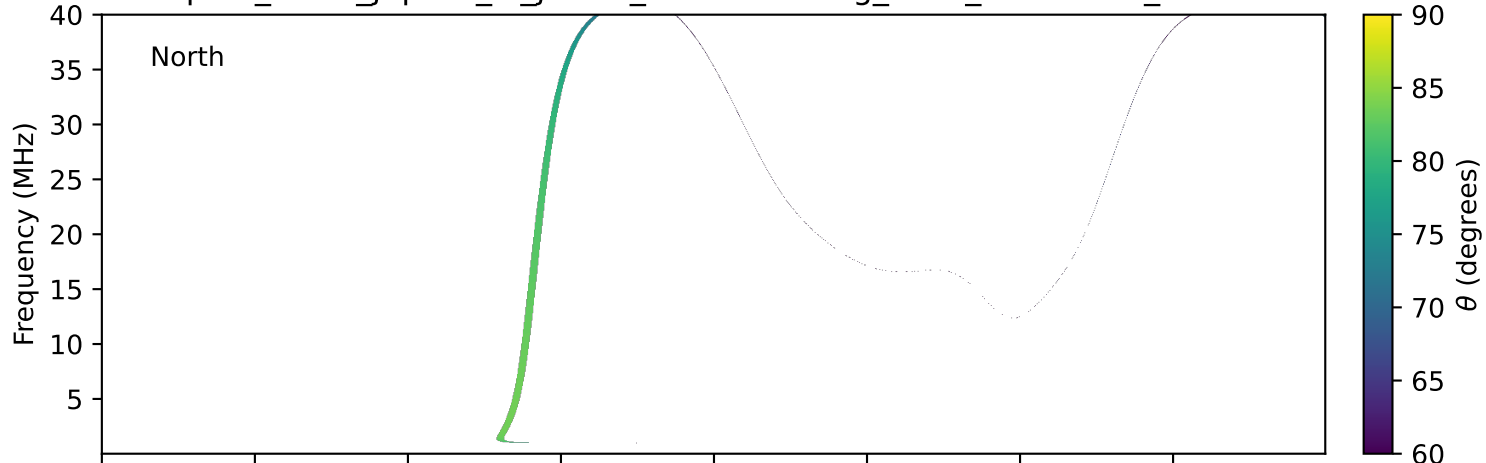
expres_earth_jupiter_io_jrm33_lossc-wid1deg_3kev_19770527_v11.cdf
