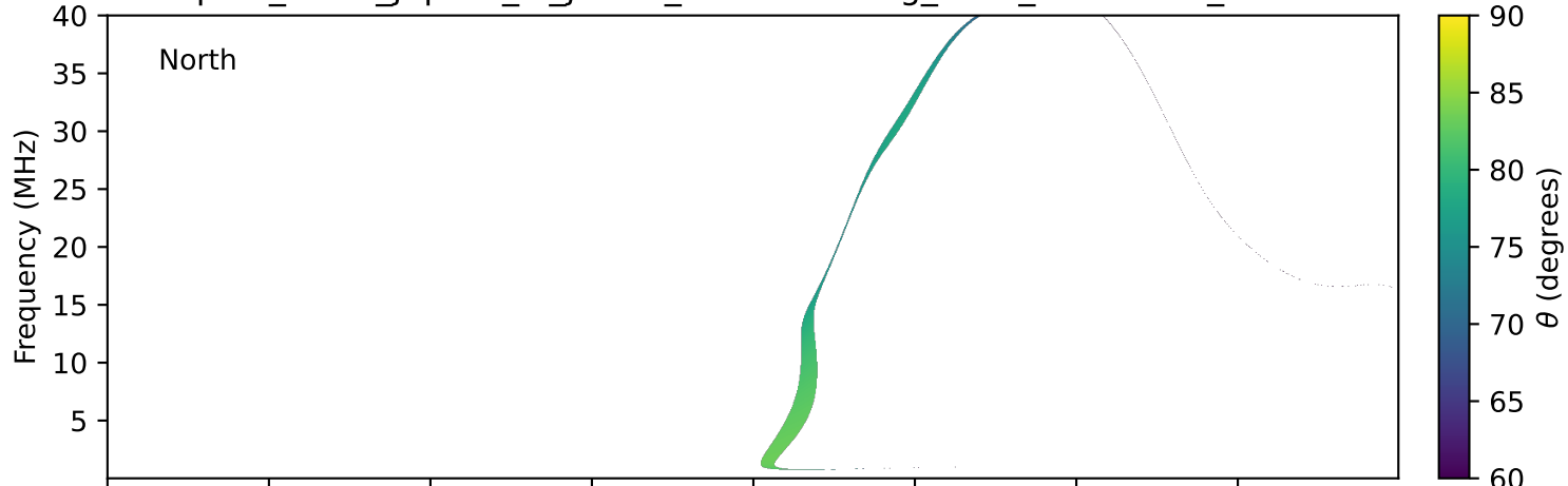
expres_earth_jupiter_io_jrm33_lossc-wid1deg_3kev_19770511_v11.cdf
