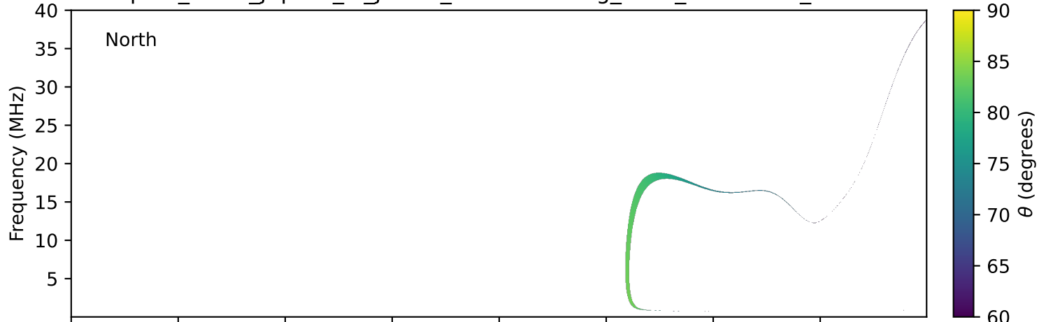
expres_earth_jupiter_io_jrm33_lossc-wid1deg_3kev_19770502_v11.cdf
