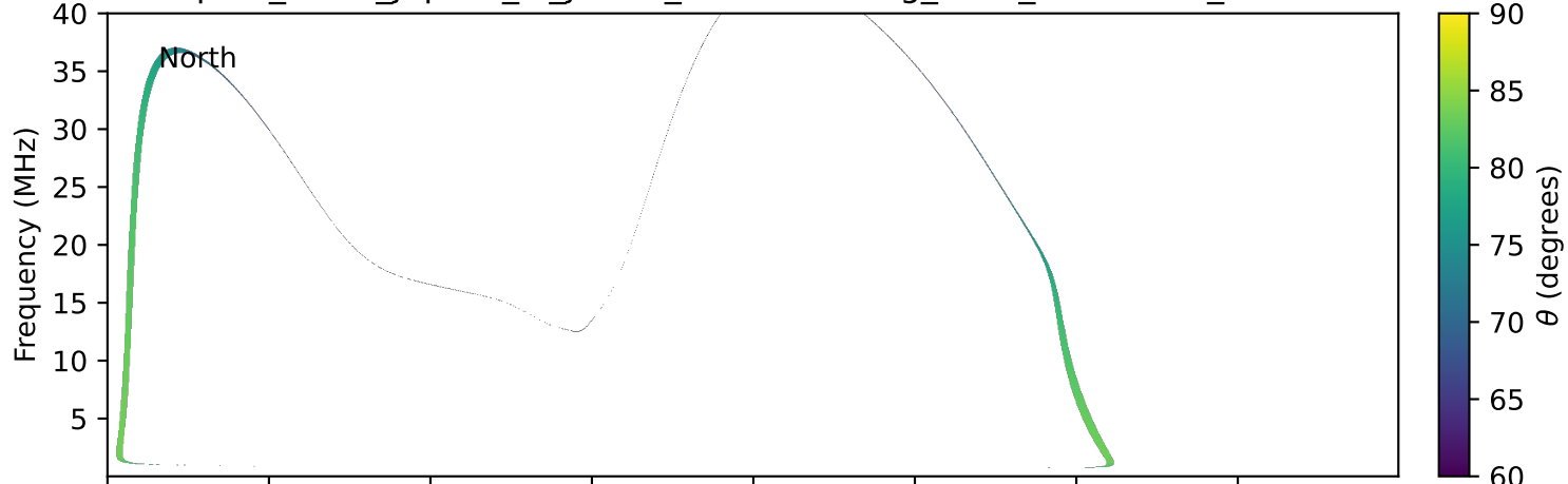
expres_earth_jupiter_io_jrm09_lossc-wid1deg_3kev_19770522_v11.cdf
