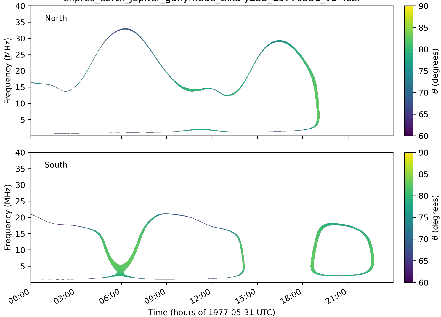
expres_earth_jupiter_ganymede_txka-y235_19770531_v14.cdf
