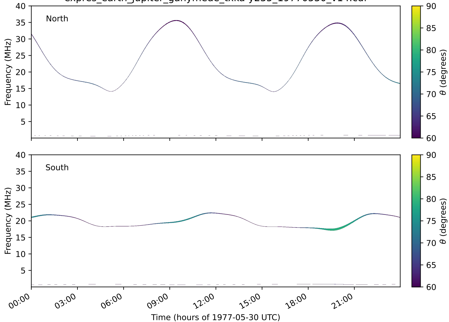
expres_earth_jupiter_ganymede_txka-y235_19770530_v14.cdf
