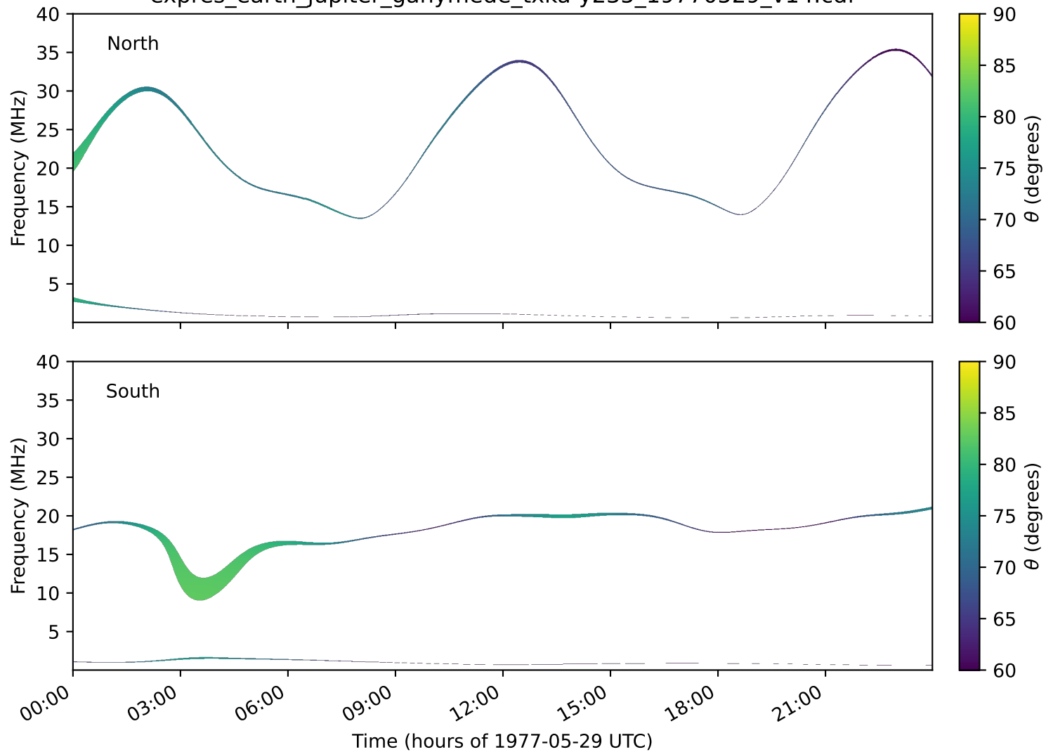
expres_earth_jupiter_ganymede_txka-y235_19770529_v14.cdf
