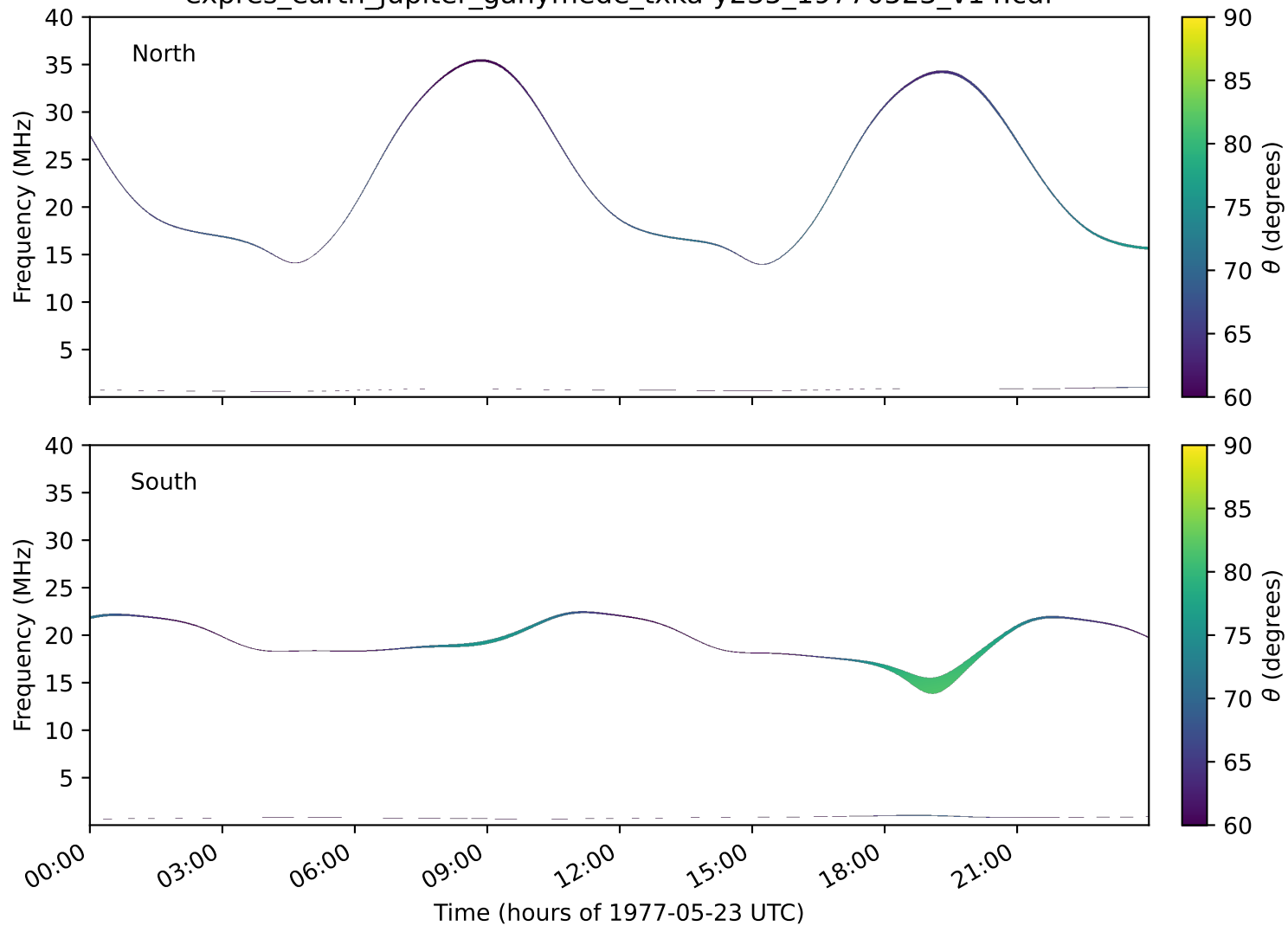
expres_earth_jupiter_ganymede_txka-y235_19770523_v14.cdf
