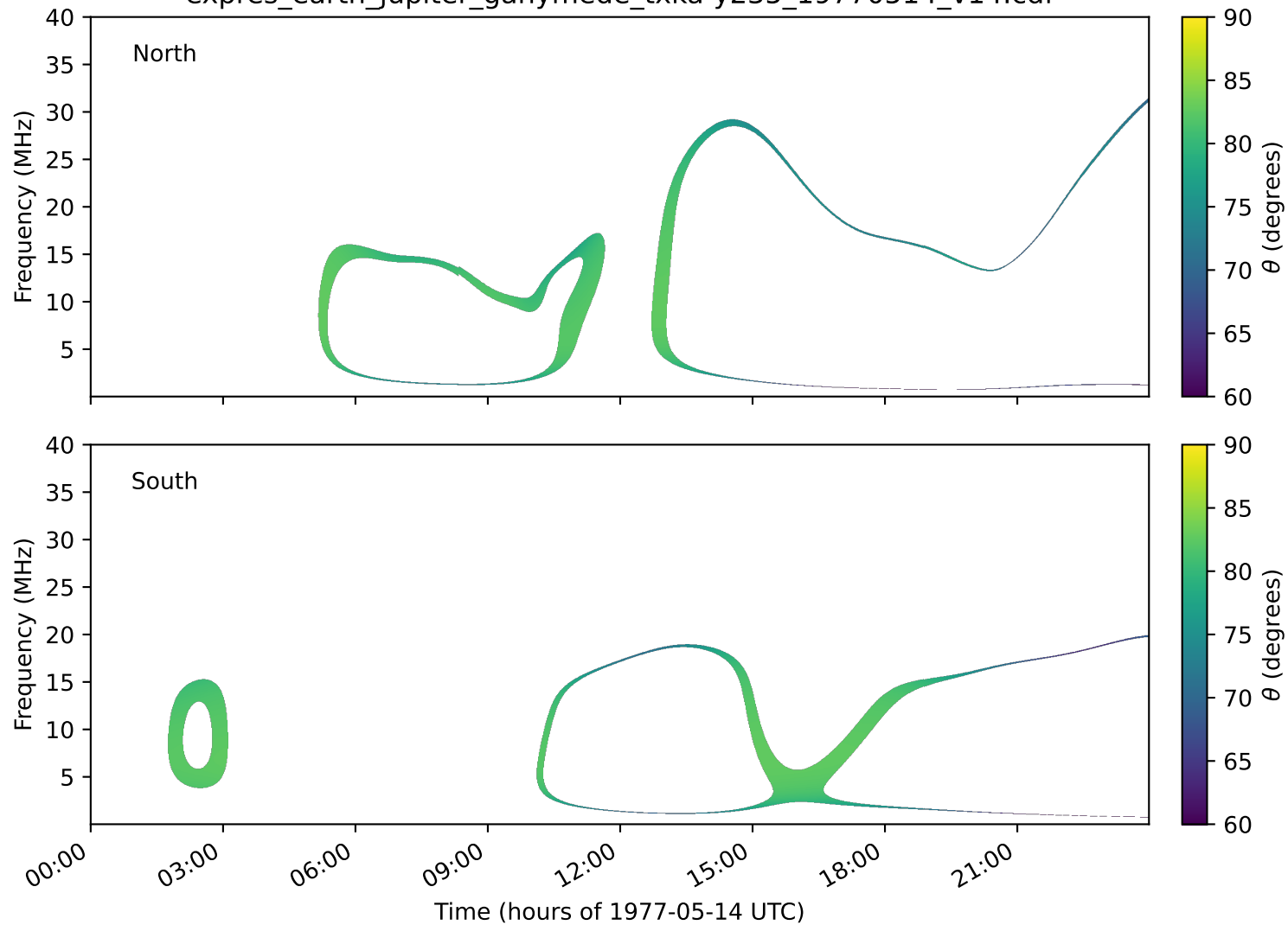
expres_earth_jupiter_ganymede_txka-y235_19770514_v14.cdf
