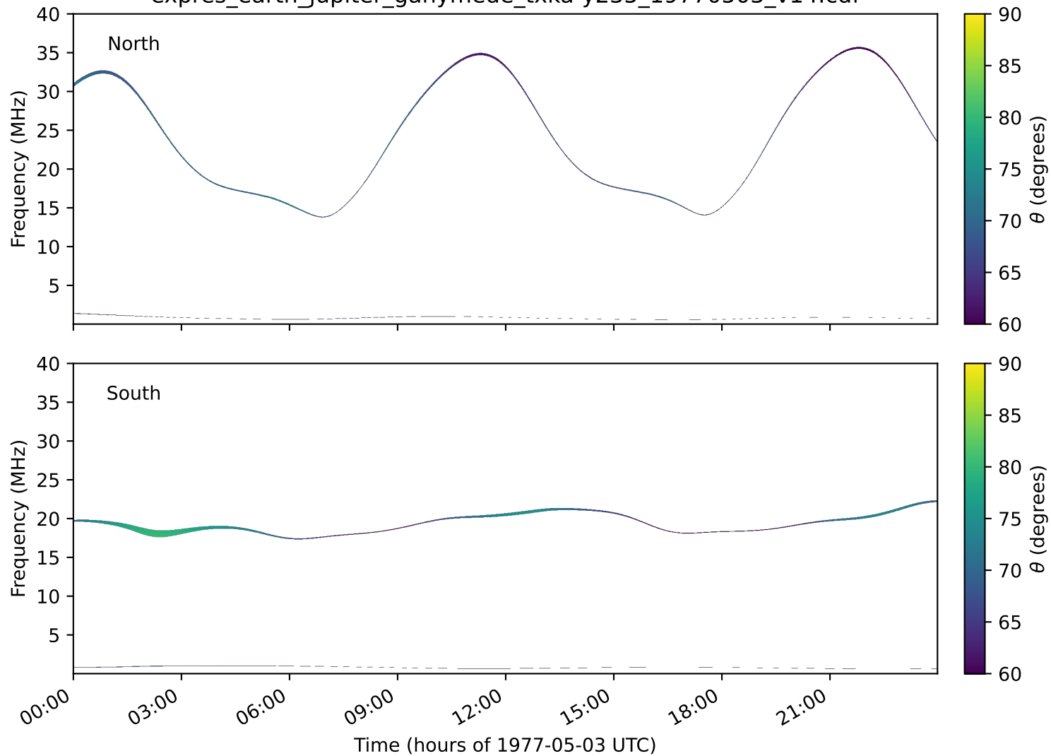
expres_earth_jupiter_ganymede_txka-y235_19770503_v14.cdf
