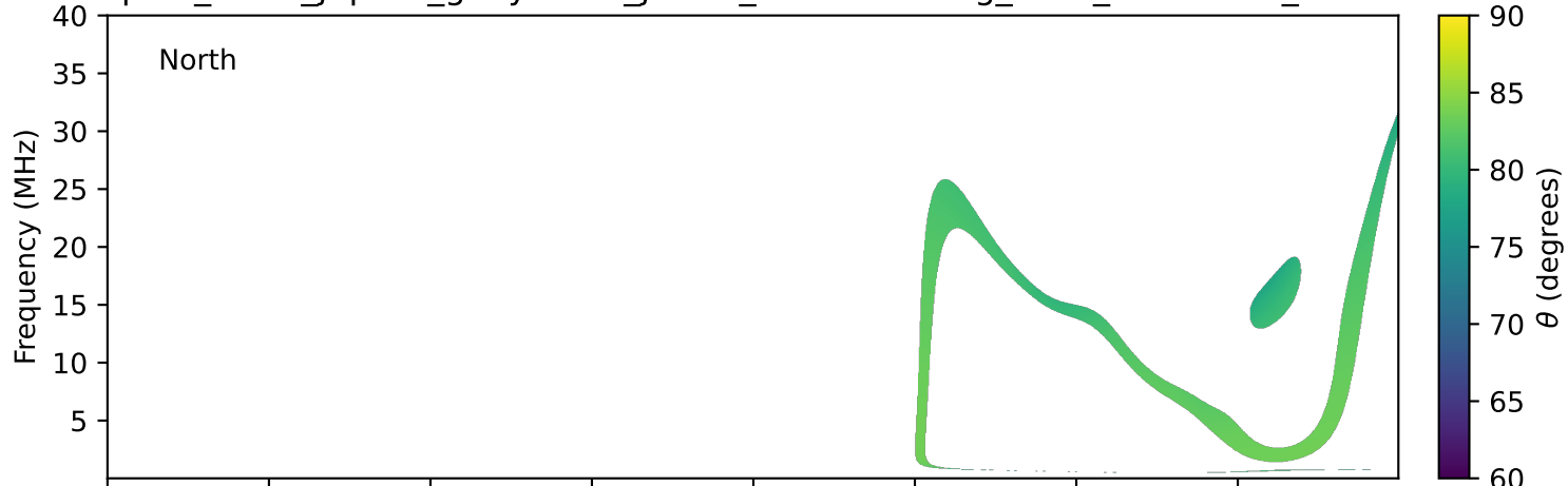
expres_earth_jupiter_ganymede_jrm33_lossc-wid1deg_3kev_19770521_v11.cdf
