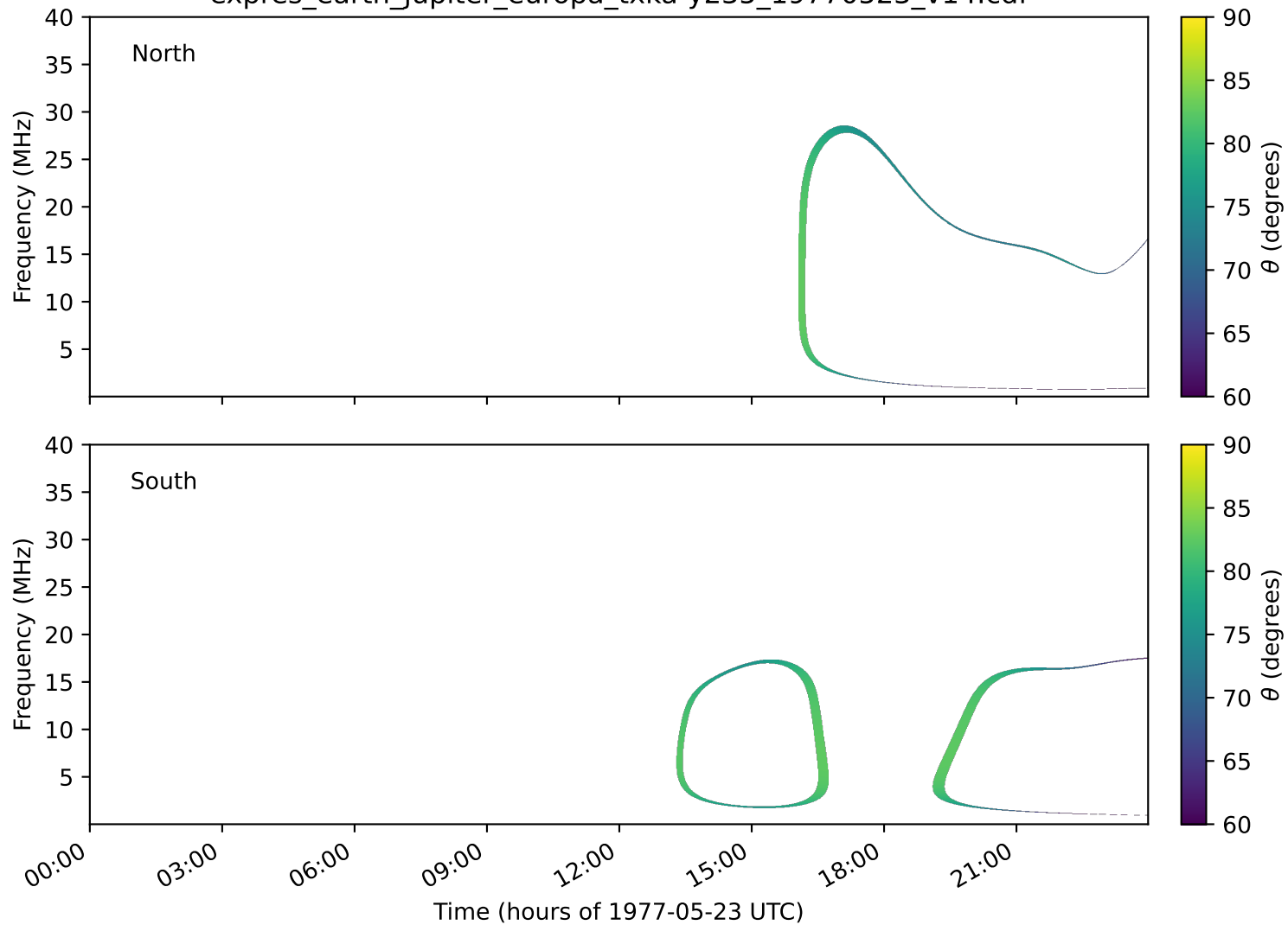
expres_earth_jupiter_europa_txka-y235_19770523_v14.cdf
