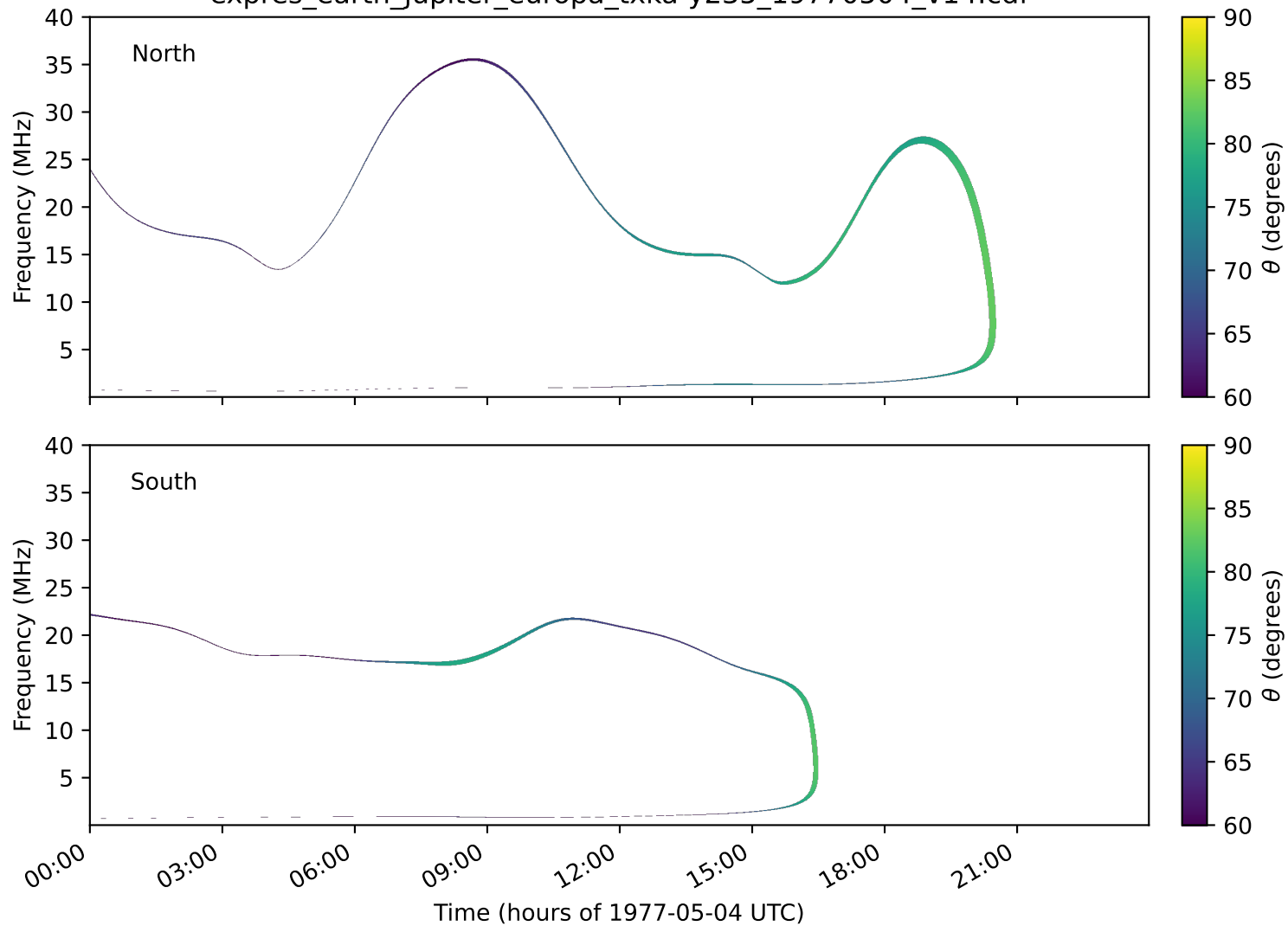
expres_earth_jupiter_europa_txka-y235_19770504_v14.cdf
