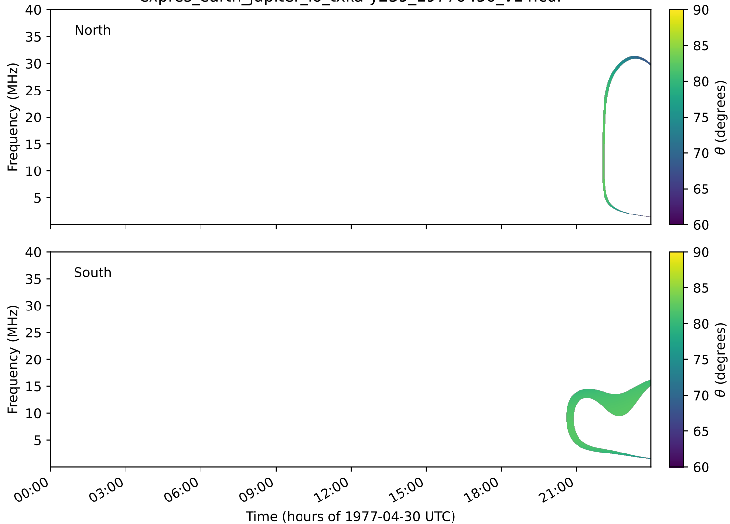
expres_earth_jupiter_io_txka-y235_19770430_v14.cdf
