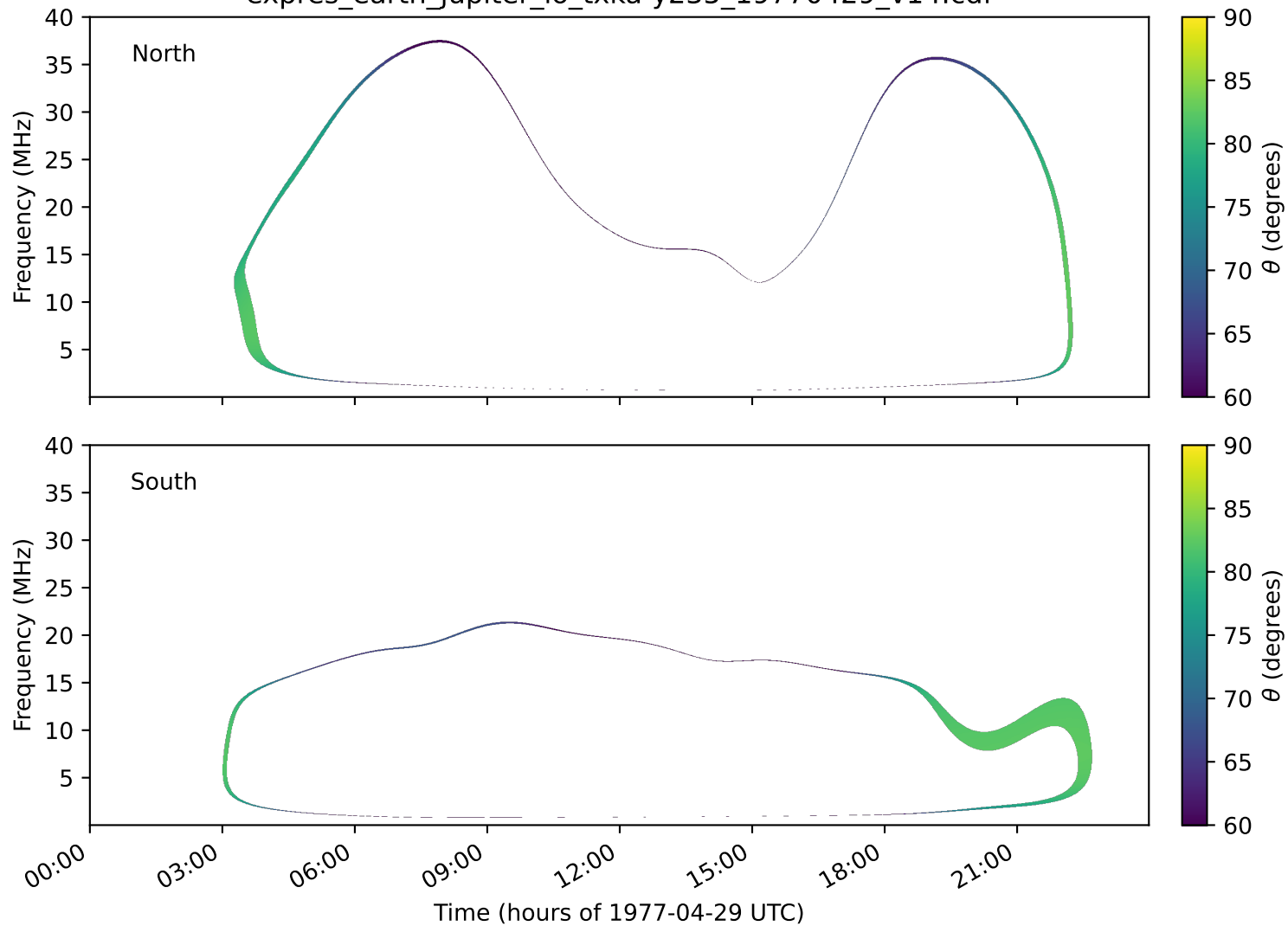
expres_earth_jupiter_io_txka-y235_19770429_v14.cdf
