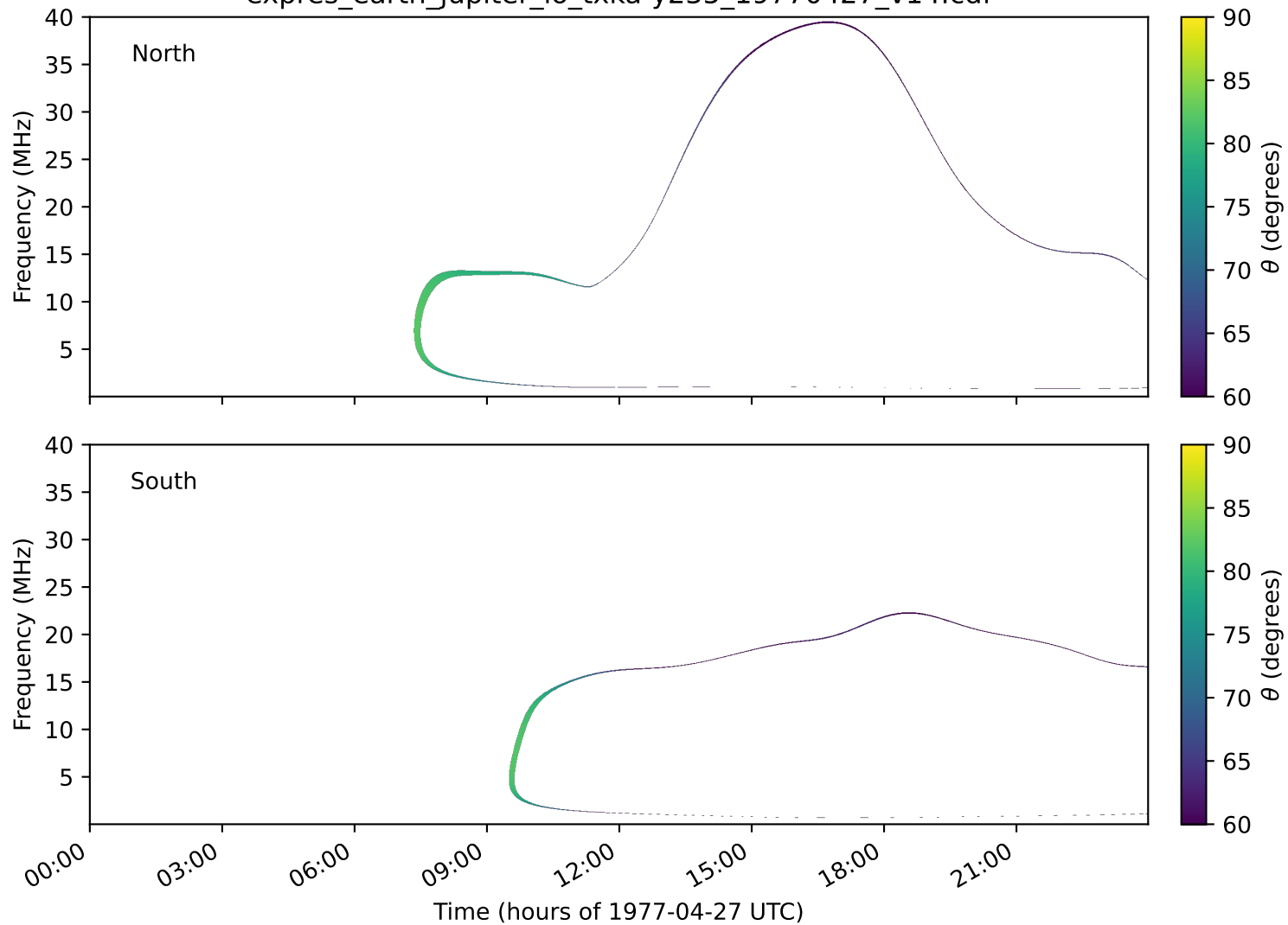
expres_earth_jupiter_io_txka-y235_19770427_v14.cdf
