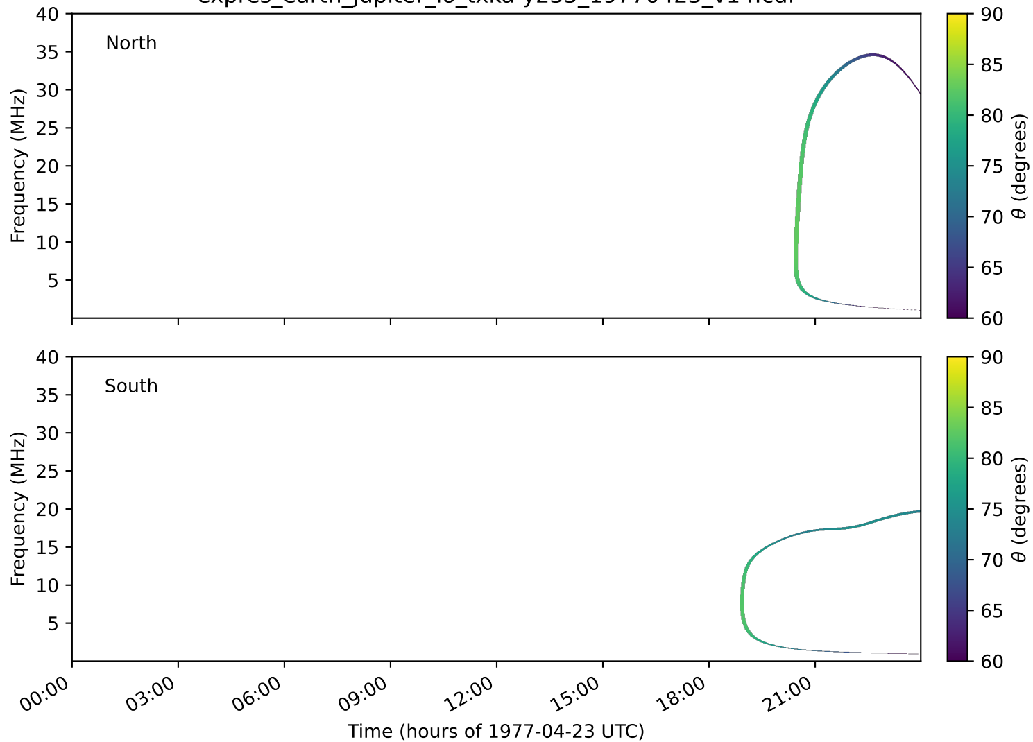
expres_earth_jupiter_io_txka-y235_19770423_v14.cdf
