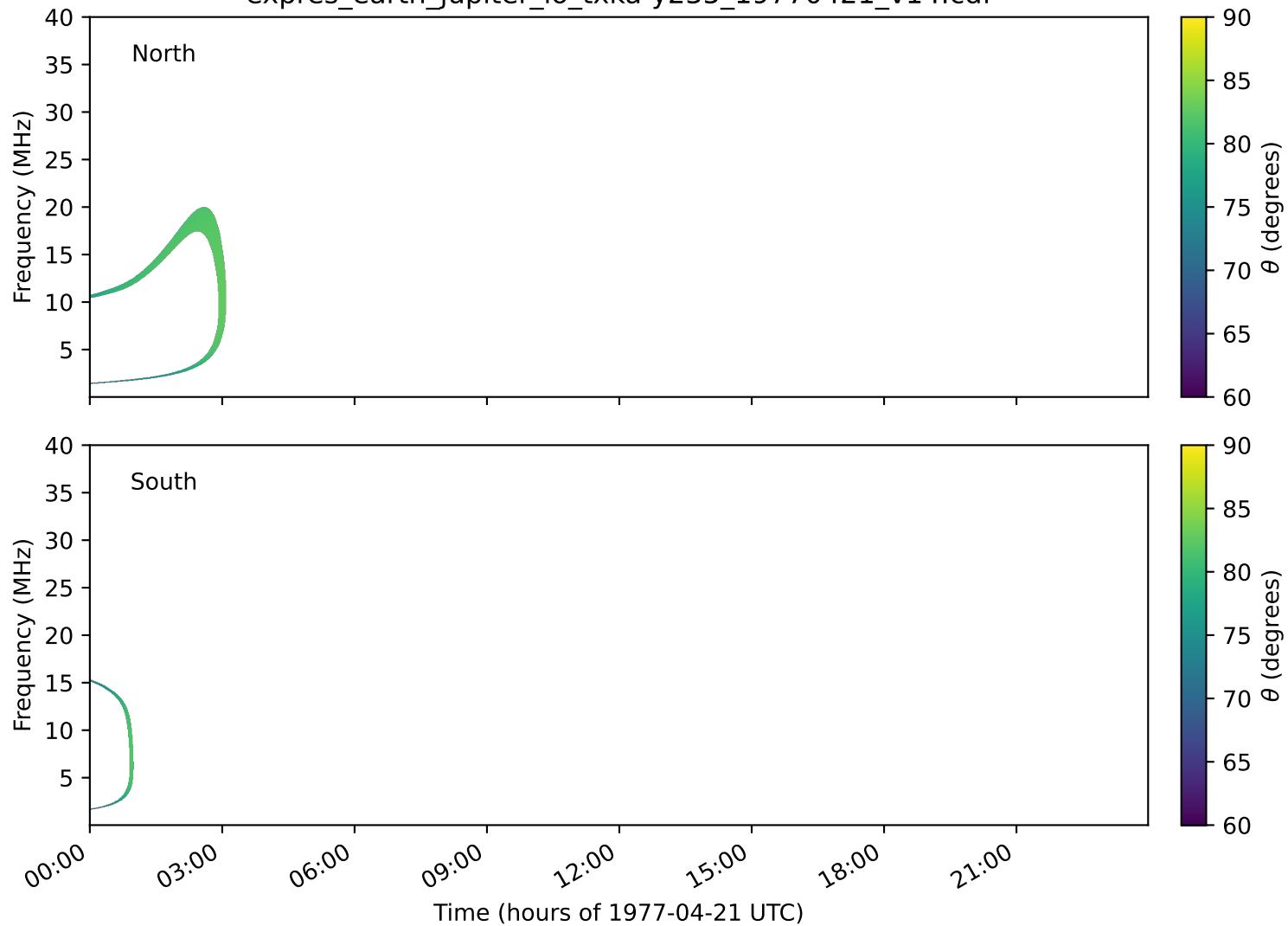
expres_earth_jupiter_io_txka-y235_19770421_v14.cdf
