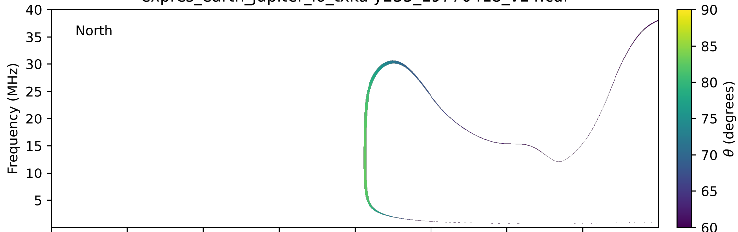
expres_earth_jupiter_io_txka-y235_19770418_v14.cdf
