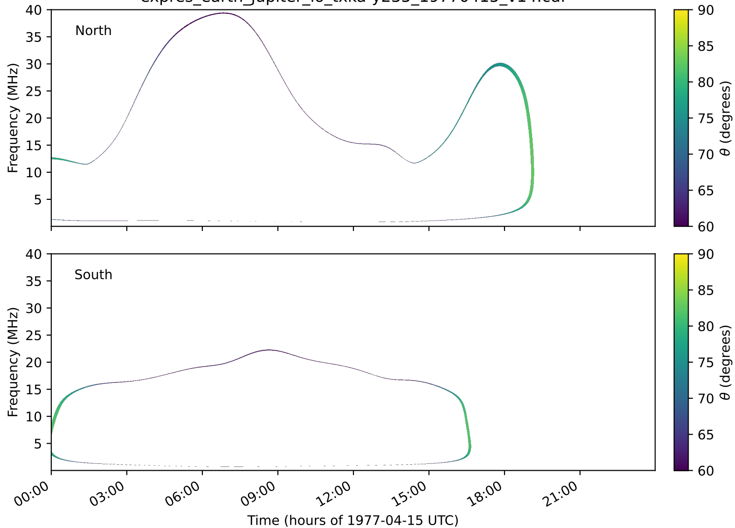
expres_earth_jupiter_io_txka-y235_19770415_v14.cdf
