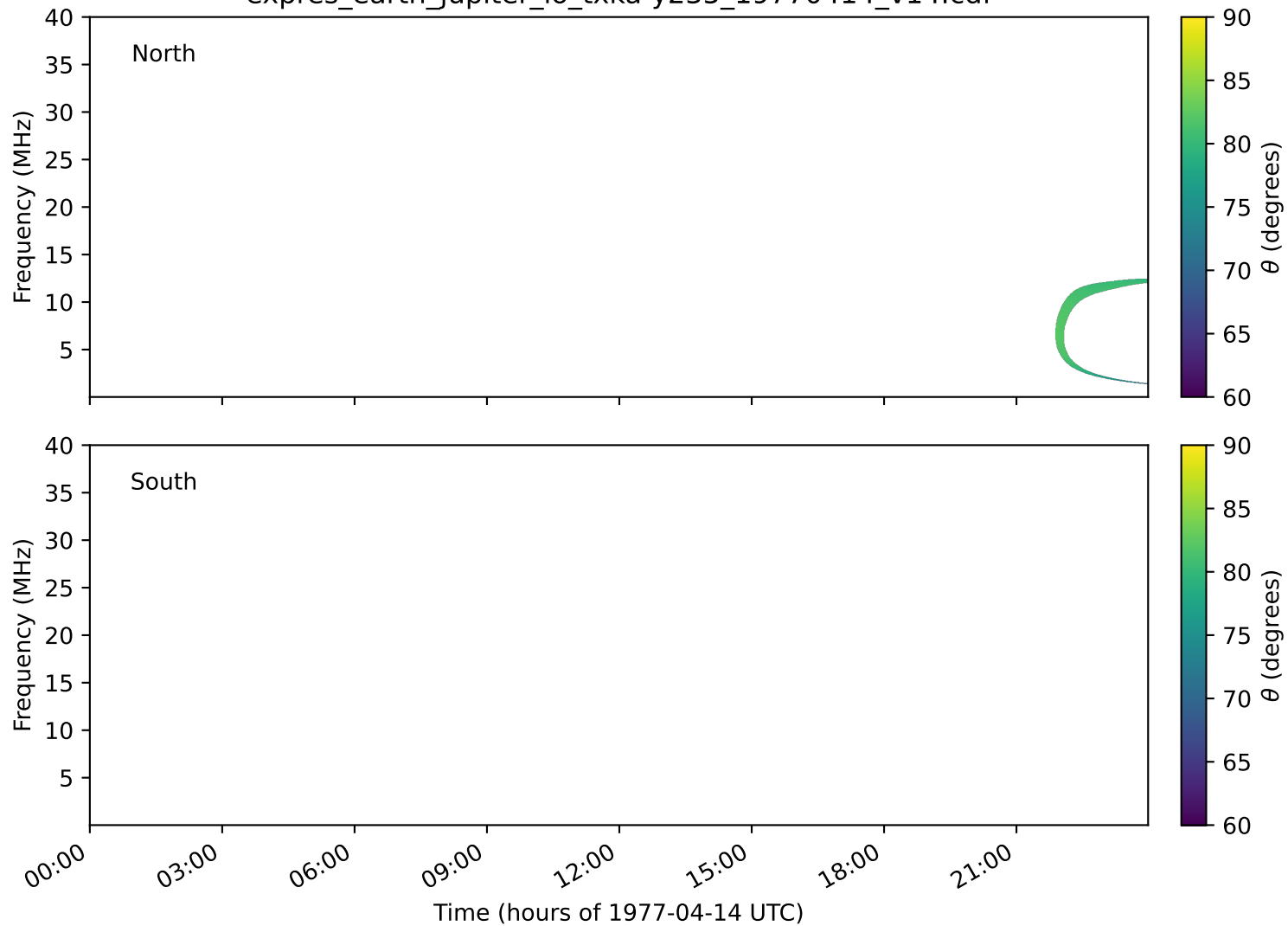
expres_earth_jupiter_io_txka-y235_19770414_v14.cdf
