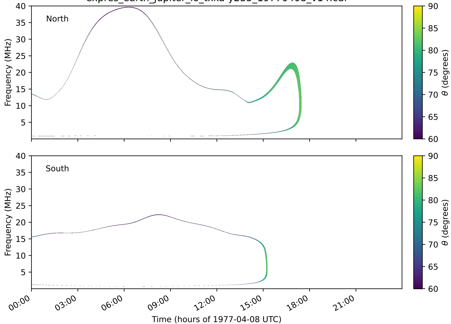
expres_earth_jupiter_io_txka-y235_19770408_v14.cdf
