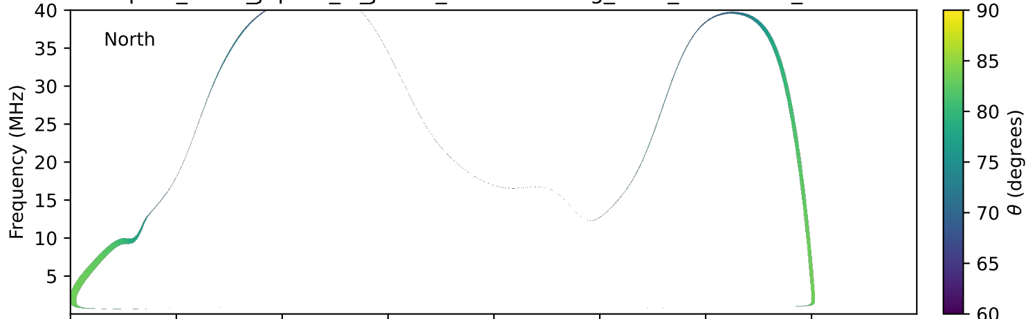
expres_earth_jupiter_io_jrm33_lossc-wid1deg_3kev_19770422_v11.cdf
