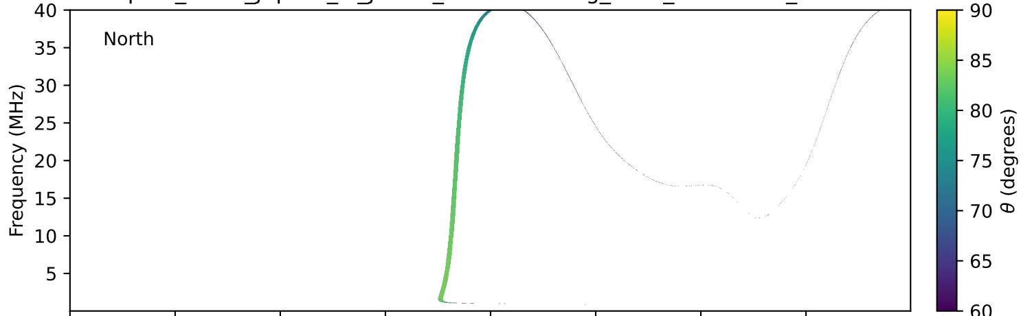
expres_earth_jupiter_io_jrm33_lossc-wid1deg_3kev_19770411_v11.cdf
