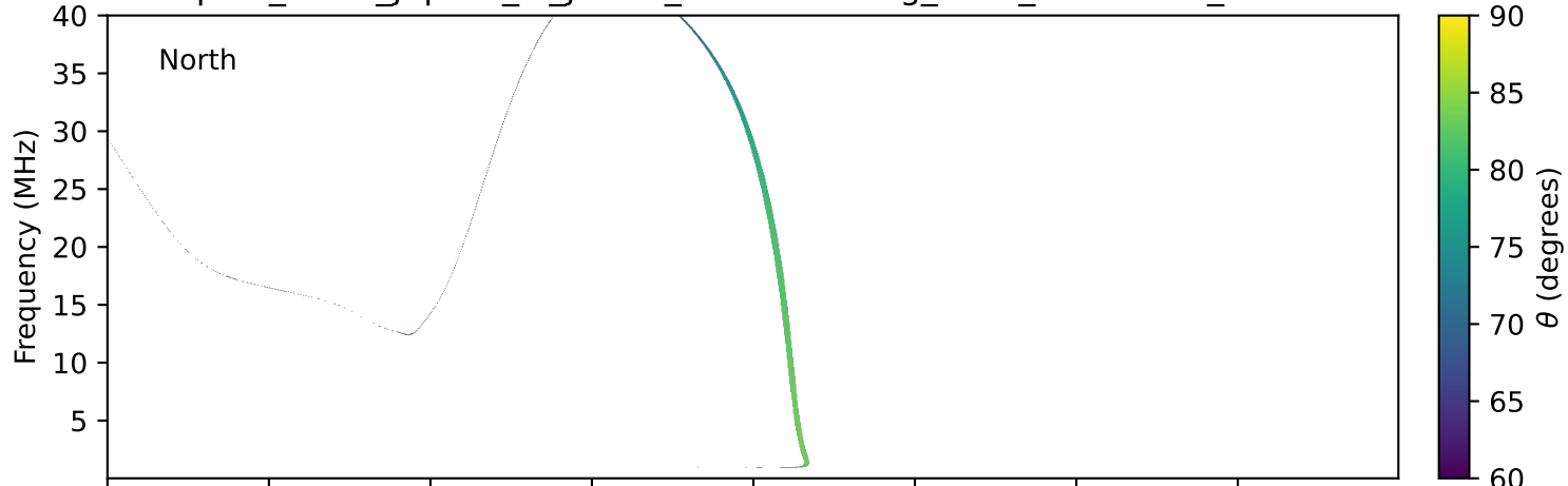
expres_earth_jupiter_io_jrm09_lossc-wid1deg_3kev_19770417_v11.cdf
