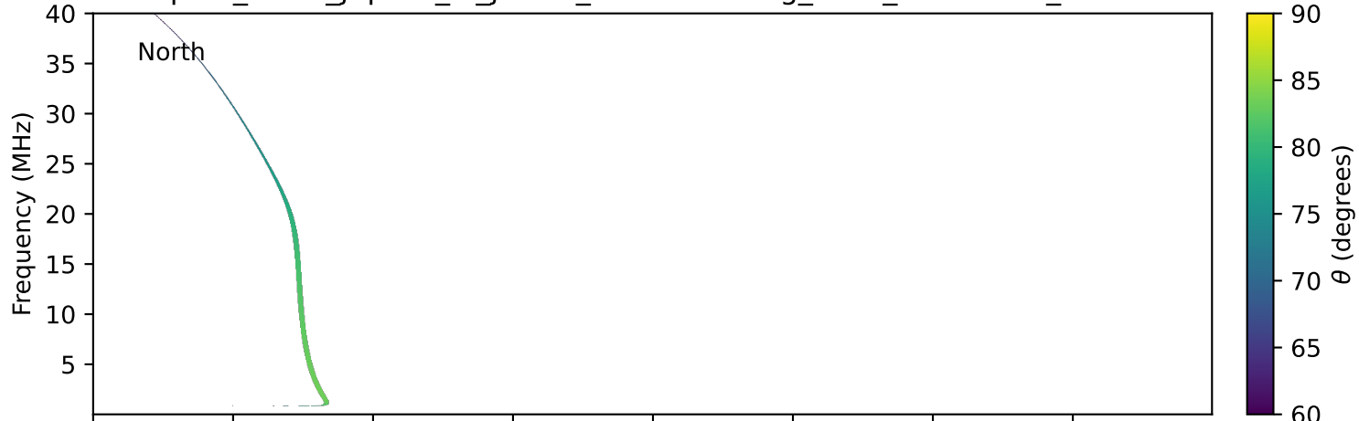
expres_earth_jupiter_io_jrm09_lossc-wid1deg_3kev_19770412_v11.cdf
