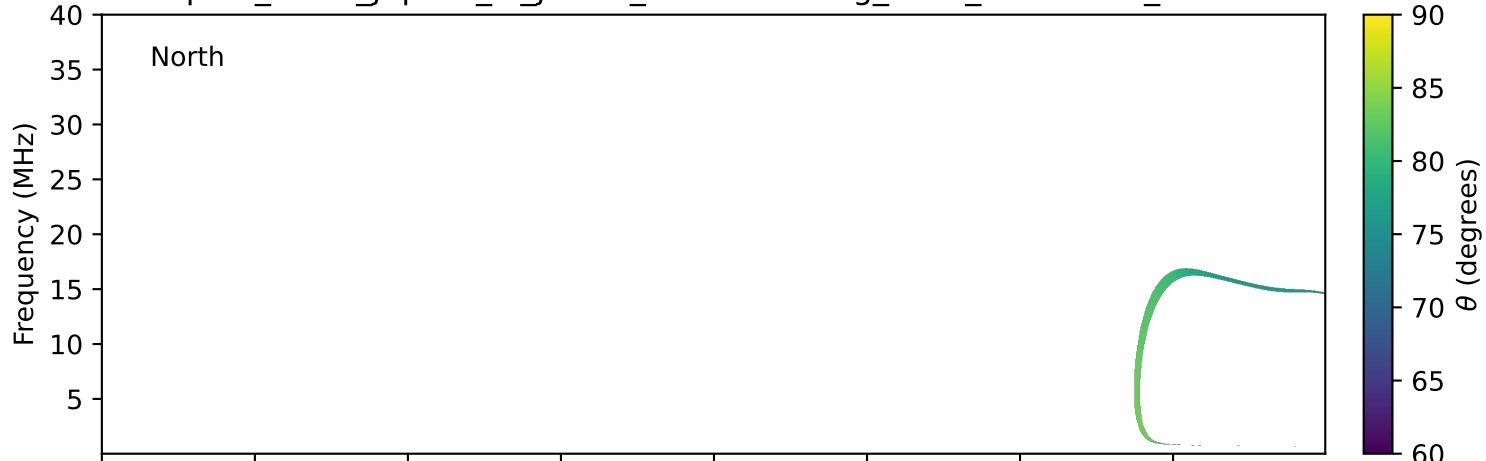
expres_earth_jupiter_io_jrm09_lossc-wid1deg_3kev_19770407_v11.cdf
