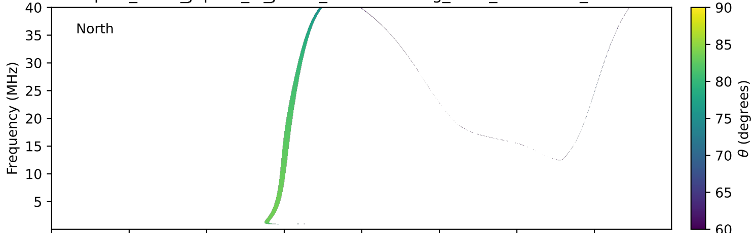
expres_earth_jupiter_io_jrm09_lossc-wid1deg_3kev_19770404_v11.cdf
