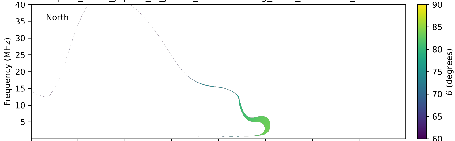
expres_earth_jupiter_io_jrm09_lossc-wid1deg_3kev_19770401_v11.cdf
