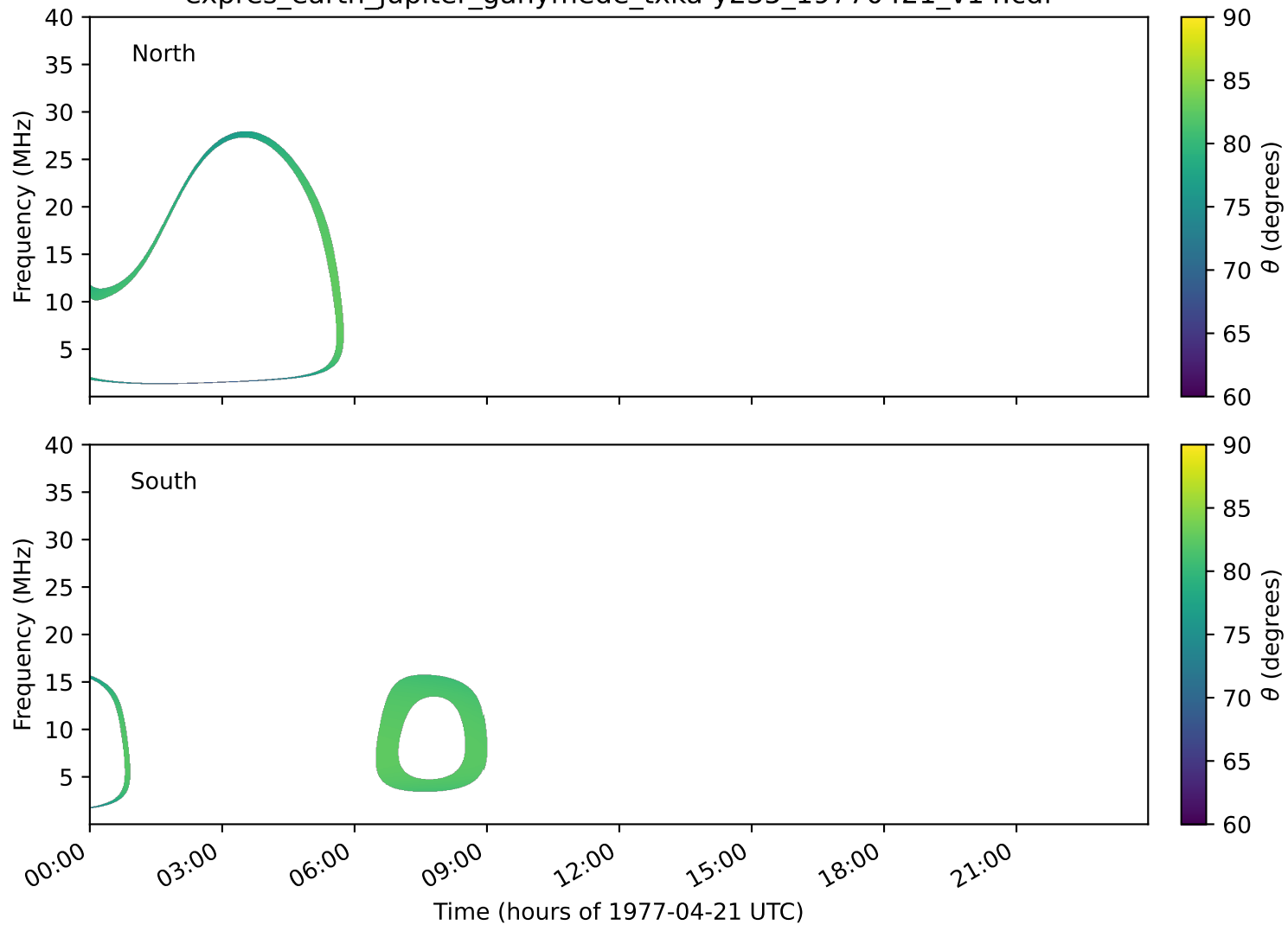
expres_earth_jupiter_ganymede_txka-y235_19770421_v14.cdf
