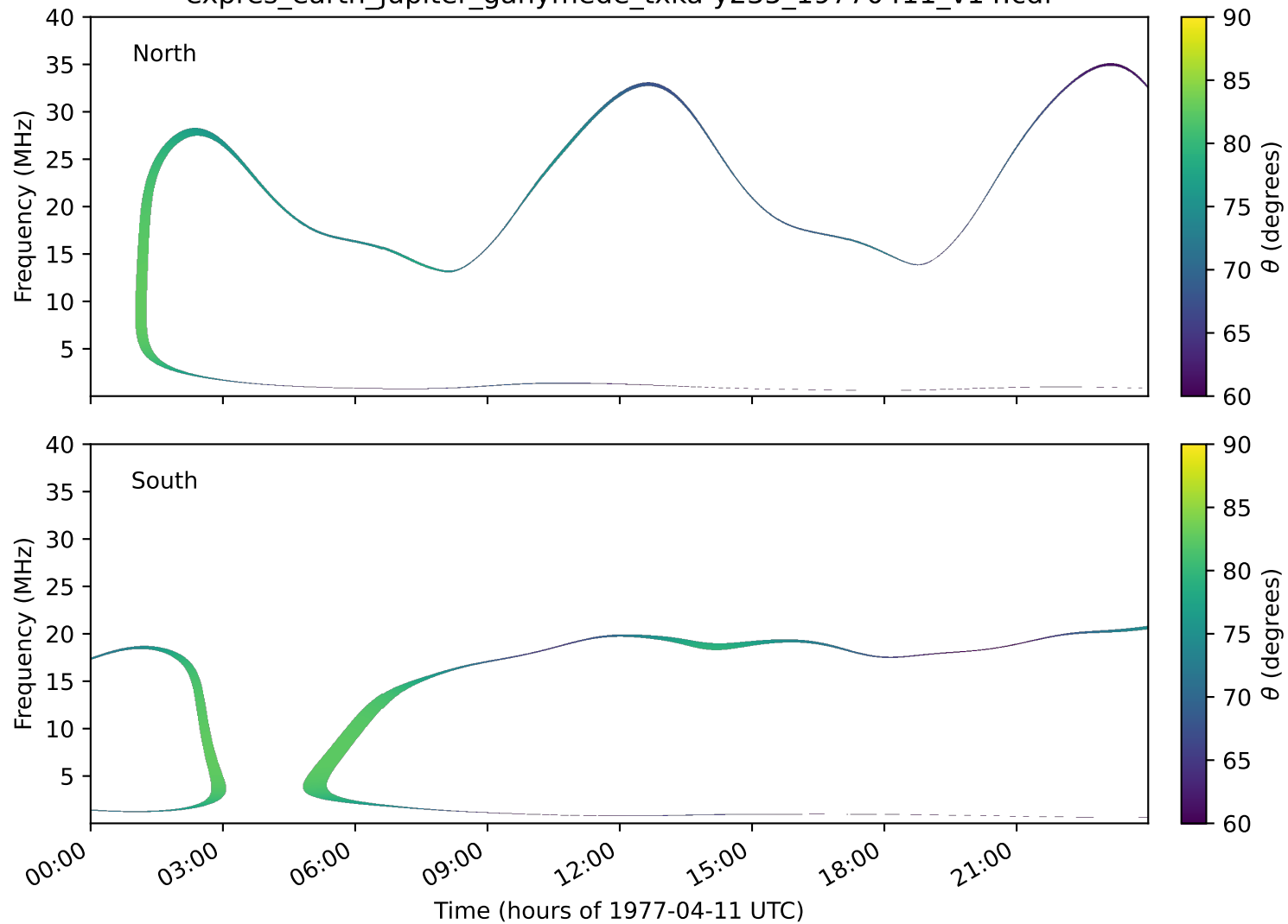
expres_earth_jupiter_ganymede_txka-y235_19770411_v14.cdf
