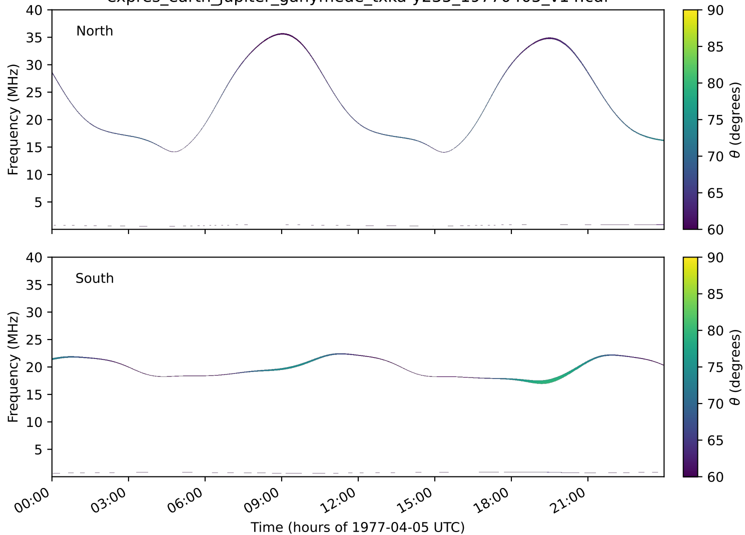
expres_earth_jupiter_ganymede_txka-y235_19770405_v14.cdf
