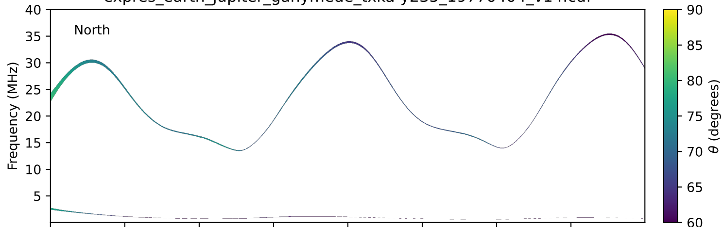
expres_earth_jupiter_ganymede_txka-y235_19770404_v14.cdf
