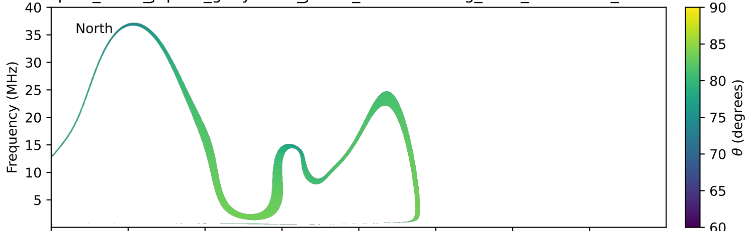
expres_earth_jupiter_ganymede_jrm09_lossc-wid1deg_3kev_19770421_v11.cdf
