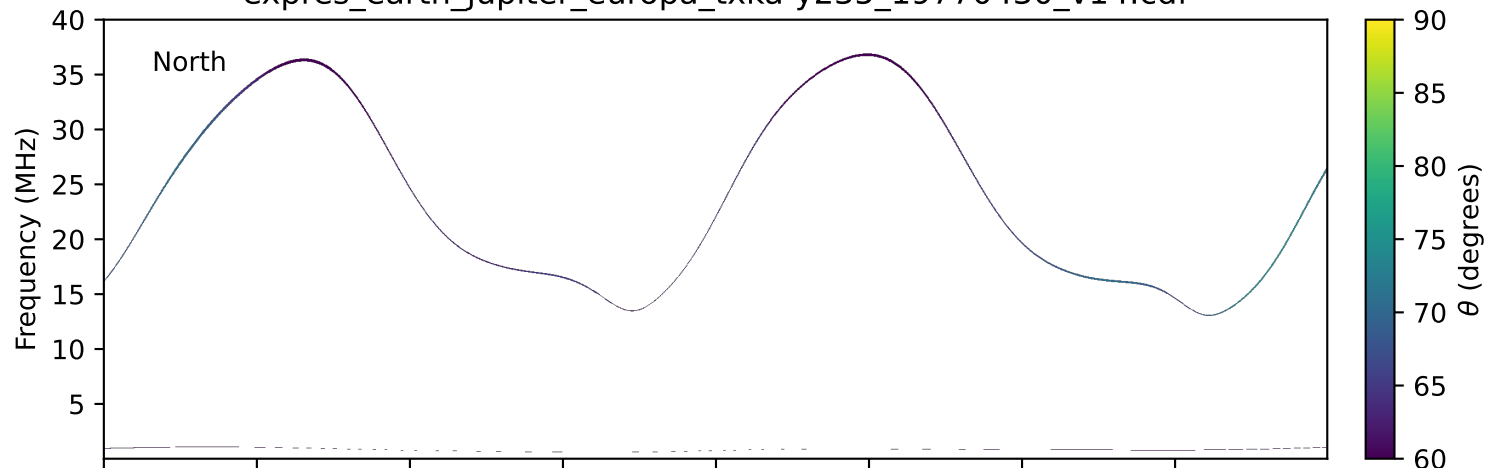
expres_earth_jupiter_europa_txka-y235_19770430_v14.cdf
