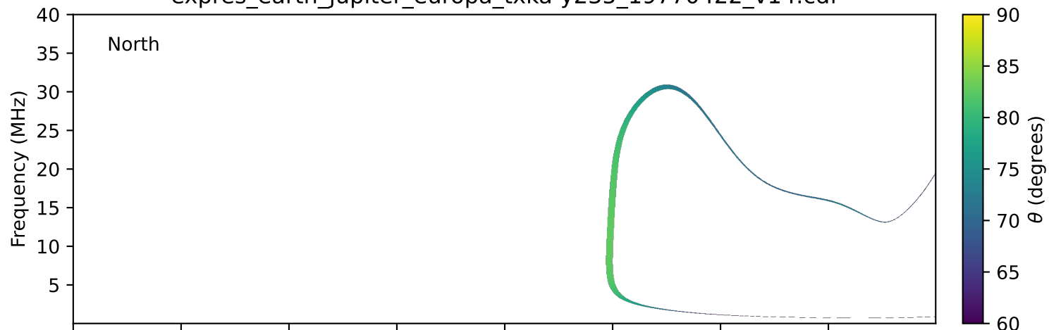
expres_earth_jupiter_europa_txka-y235_19770422_v14.cdf
