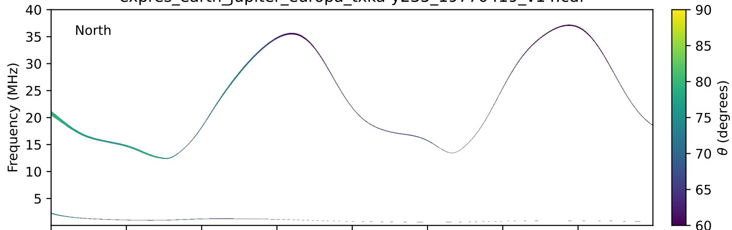
expres_earth_jupiter_europa_txka-y235_19770419_v14.cdf
