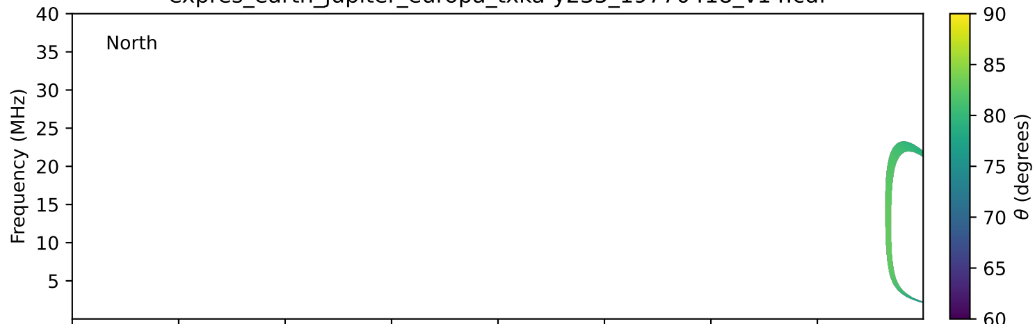
expres_earth_jupiter_europa_txka-y235_19770418_v14.cdf
