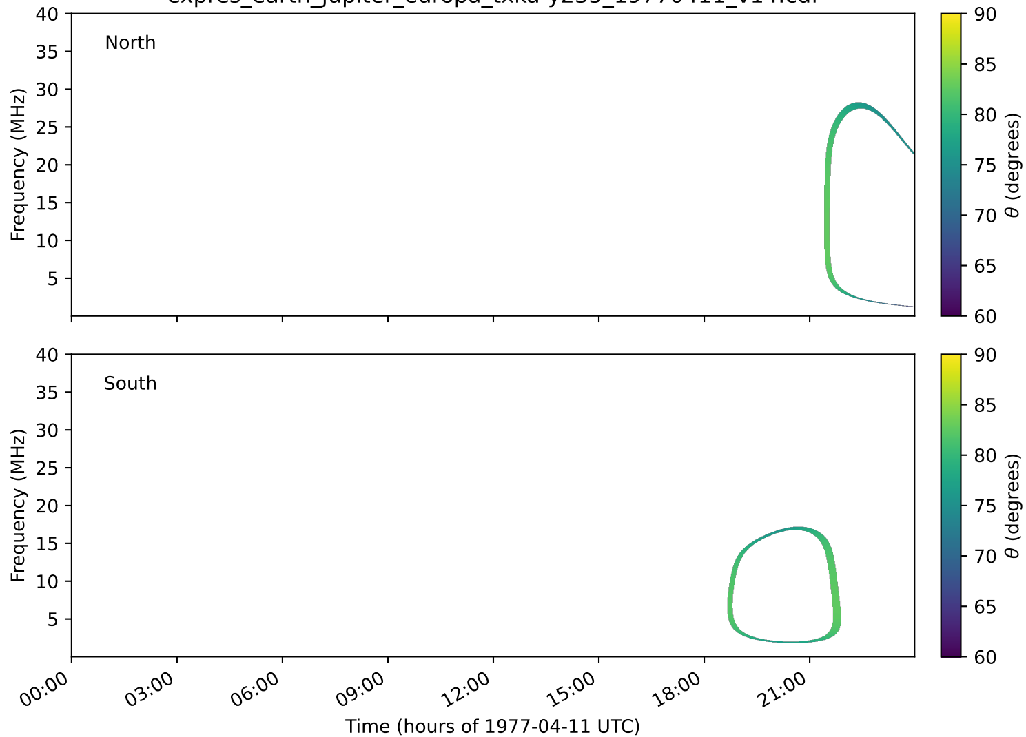
expres_earth_jupiter_europa_txka-y235_19770411_v14.cdf
