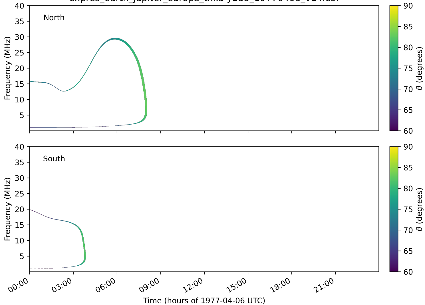
expres_earth_jupiter_europa_txka-y235_19770406_v14.cdf
